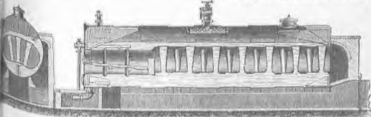
16. Λέβης Galloway.
