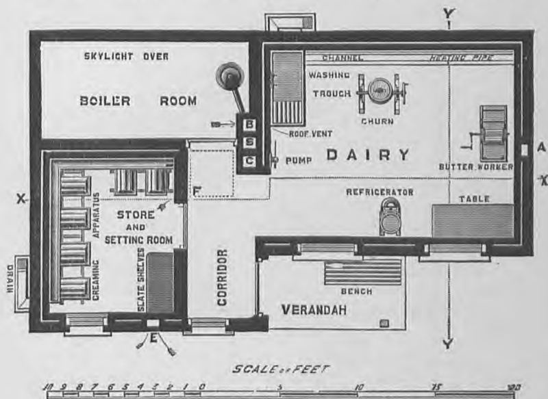
FIG. 29.—PLAN OF BUTTER DAIRY FOR A FARM OF UNDER 100 ACRES.
