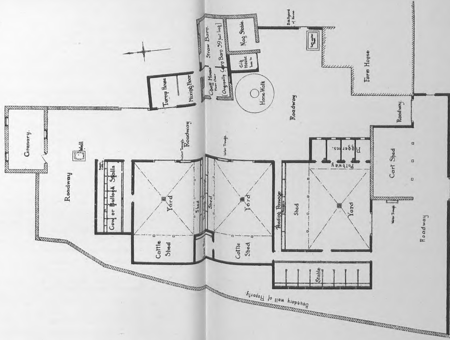
FIG. 7. PLAN OF OLD HOMESTEAD REMODELLED Nº 2.
