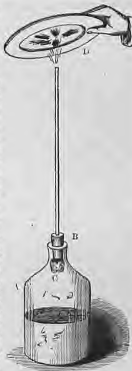
Fig. 230. Marsh's Test. A , Bottle containing zinc and dilute sulphuric acid and the suspected fluid, B , Cork and tube, or clean tobacco-pipe fitted through cork, and having some clean, dry cotton-wool, C , lightly tied at the bottom of the cork, to stop the moisture which condenses in the pipe and spoils the experiment. D , Plate covered with black stains of arsenic; in one or two seconds an arsenic mirror is obtained, and if the plate is held over the flame for a longer time, the indication may be lost.
