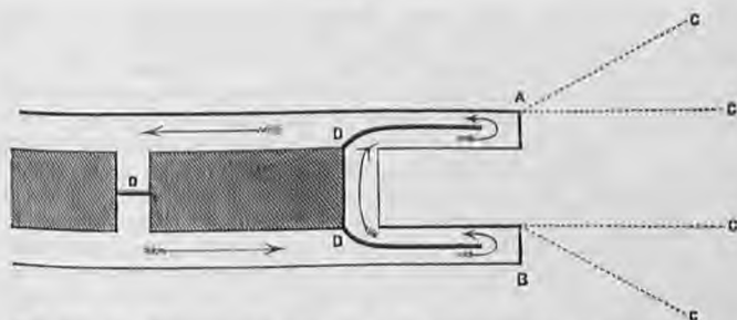
Fig. 187. The Pillar and Stall System. A, B. Main working-places. C, C, C. Exploring bore-holes. D, D, D. Brattices, or timber partitions to confine the air (shown by the arrows) in its proper channel, and make it sweep round the places where the men are working at A, B. The shaded parts represent the pillar left to support the roof.
