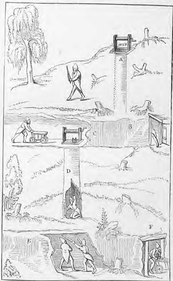
Fig. 149. A B. Main shaft. C B. Gallery heavily timbered. D. Shaft connecting the galleries with each other, called a winze. E F. Gallery timbered. (Agricola.)
