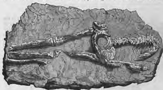
Fig. 190. Human Remains embedded in an Alluvial Mass.
