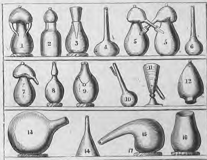
Fig. 75. 1. A Pellican, or circulating vessel. 2. Another vessel of circulation. 3. An infernal glass. 4. A Matraces, or bout head, with a flat bottom. 5, 5. A Troir, or double Pellican. 6. A Matraces, or bout head. 7. An Alimbiick made of one peece, or a head and body joyned at the first making. 8. The Phylosopher's egg. 9. A double egg, or one within another. 10. A little Matraces. 11. A separating glass. 12. A blind head, or a head without a beak. 13. A receiver. 14. A glass funnel. 15. A Cornuc, or a retort. 16. A Curcabit, or a body for an alimbiick. 17. A ring, or round route of straw, to hold glass vessels.
