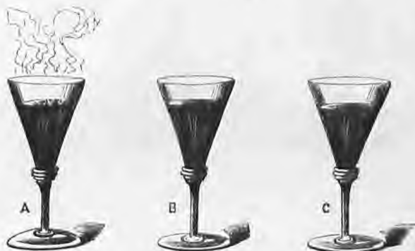
Fig. 117. A. Copper turnings or sham nugget in nitric acid. B. Glass containing gold leaf and nitric acid. C. Glass containing gold leaf and hydrochloric acid. When the contents of A and C are mixed together, the sparkling fragments of gold leaf soon disappear.
