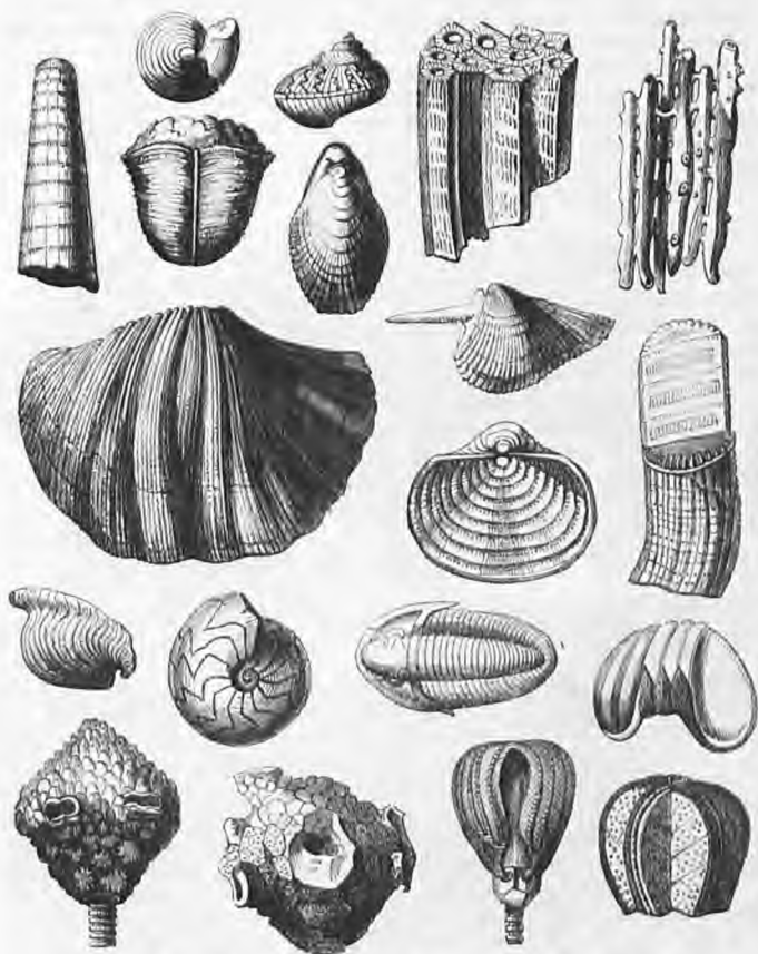
Fig. 26. Fossils of the Mountain Limestone and Carboniferous Shale.
