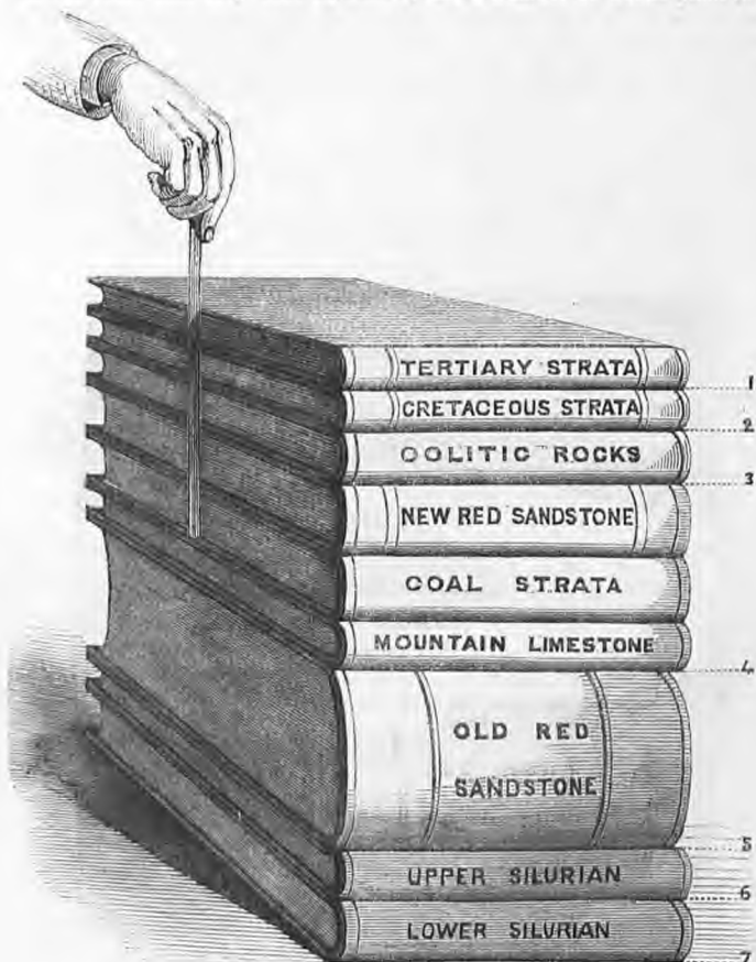
Fig. 24. The books represent a thickness of about 5 miles, and the hand holding the stick indicates the great depth of the Coal Strata.
