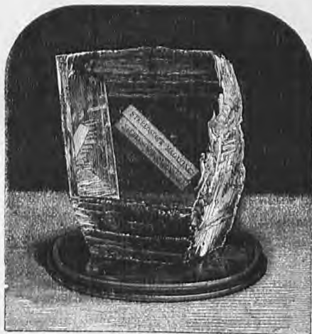
Fig. 237. Immense specimen of Calc Spar, called Double-Refacting Spar, from Professor Tennant's collection. Proportions, nine inches high, seven inches and three-quarters broad, five inches and a half thick; estimated value, one hundred pounds.
