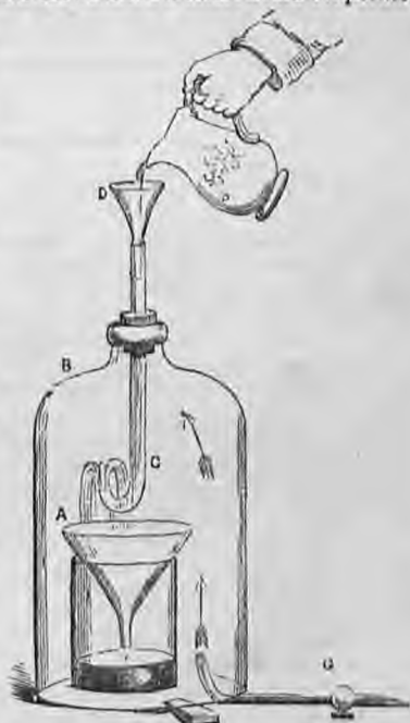
Fig. 170. A. Funnel and filter containing the sulphide of copper, &c. B. Gas jar fitted with a cork and glass tube in neck; the tube is bent round at C, so that the coal gas may not escape. p. The funnel by which the water is poured in to wash the sulphide of copper, and by turning the beaker round that supplies the funnel, every part of the filter may be washed. G. Gas-pipe connected with the coal-gas fittings. The arrows denote the entry of the gas.
