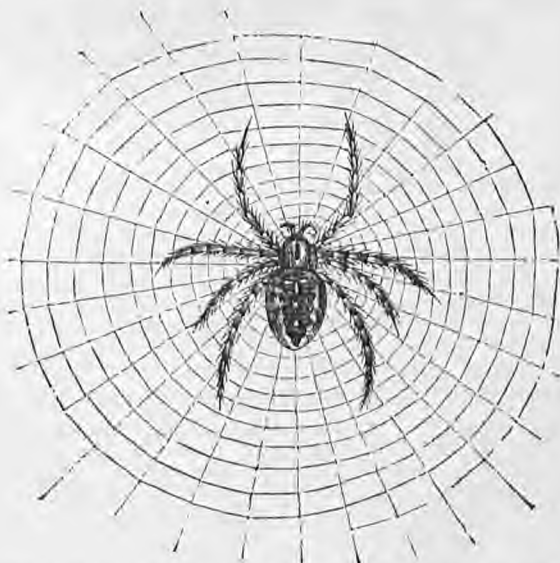
Fig. 242. The Spider's Web upon which dew deposits, and, when lighted by a sunbeam, produces the beautiful prismatic colours of the iris, the origin of the word Iridium.
