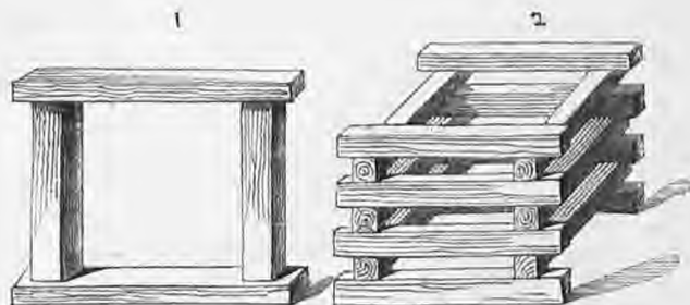
Fig. 195, Timber Supports used in Mines. No. 1, Props and planks. No. 2, A "chock" of timber for supporting the roof of a main way.
