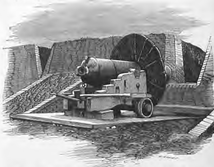
Fig. 219. Eight-inch Gun on Rear-chock Carriage, covered by the Russian Mantelet.
