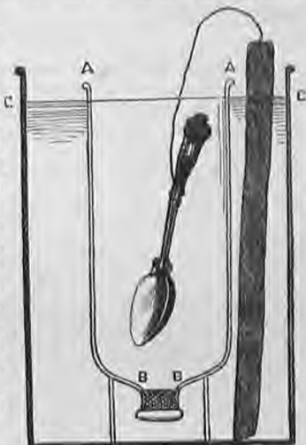
Fig. 126. A A. Inverted gas jar. B B. Neck of jar closed with linen and clay; the jar contains the solution of gold. C C. The outer earthen vessel containing the solution of ferrocyanide of potassium and chloride of sodium; also the plate of zinc not amalgamated, and attached by a platinum wire to the spoon.
