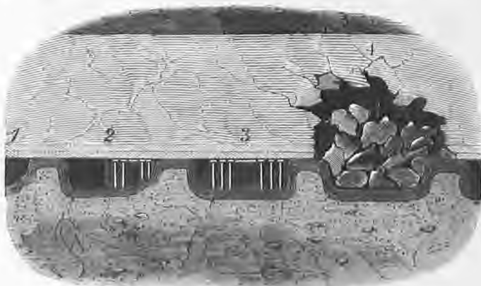
Fig 55. A Creep, and Cause of Thurst.
