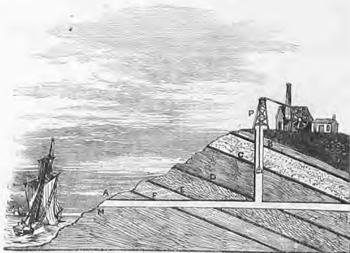
Fig. 33. "A Day Level."
