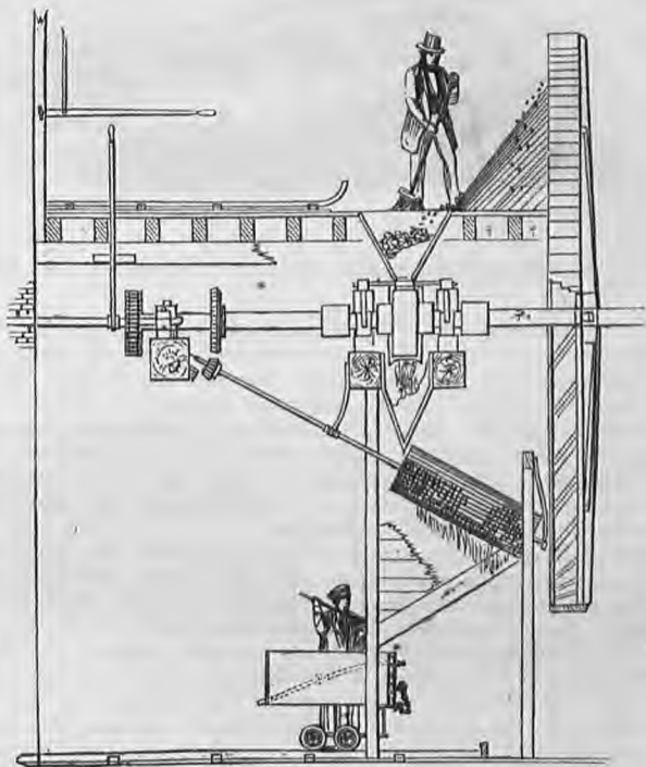
Fig. 112. A Cornish Crushing Machine worked by a Steam Engine.
