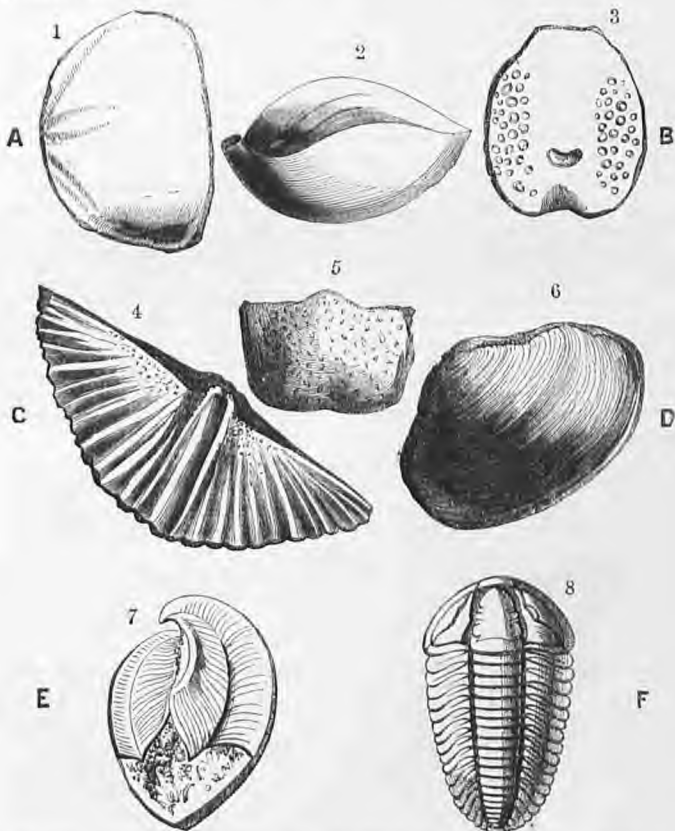
Fig. 110. A to B. Australian Fossils of the older Tertiaries. 1. Echinolampas. 2. Spatangus. 3. Terebratula Compta. — c to D. Australian Fossils of the Upper Palæozoic or Silurian Rocks. 4. Spirifer. 5. Productus. 6. Pachydomus. — E to F. Lower, or older Palæozoic Fossils. 7. Pentamerus. 8. The Trilobite.
