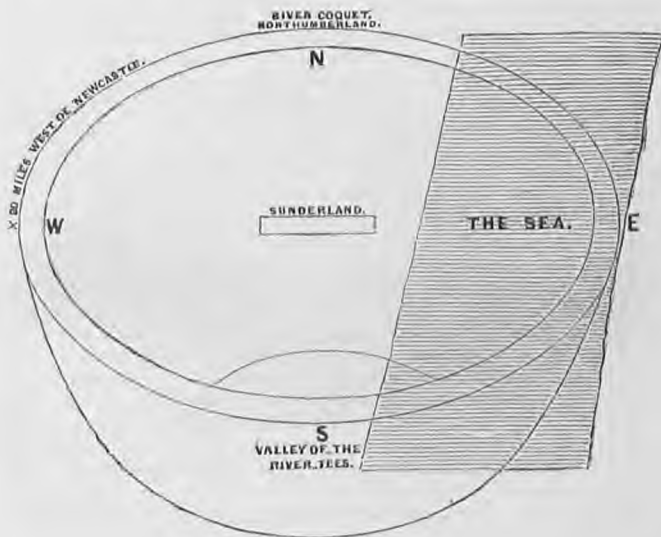
Fig. 18. The Great Coal Basin in the N.E. Corner of England.
