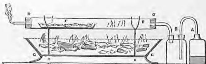
Fig. 221. A. Hydrogen generator. B. Chloride of calcium bottle, for drying the gas. C, D. The Bohemian-glass tube, containing the chloride of aluminium at E, and the tray of sodium at F. G G. The chafing-dish, containing burning charcoal. H, H. Wire supports for the tube.
