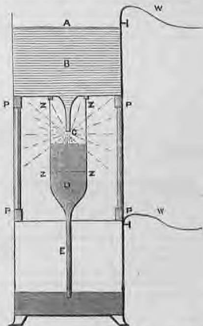
Fig. 189. Way's Mercurial Electric Lamp. A. Upper iron cistern containing u , the mercury, which falls slowly, in a fine stream, through the minute aperture, c , on to a little cup not shown, because invisible when the light is produced, and placed in the glass tube z z z z , connected with the lower iron cistern, e . The two metallic cisterns are cut off from conducting communication with each other by the non-conducting material inserted at the pillars p p . W, W . Wires passing to the voltaic battery.
