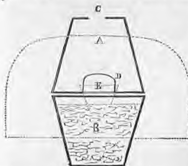
Fig. 139. A B. Black-lead crucible. C. The upper opening. D. The lower opening. E. The cupel. The dotted semicircle represents the position of the furnace door.
