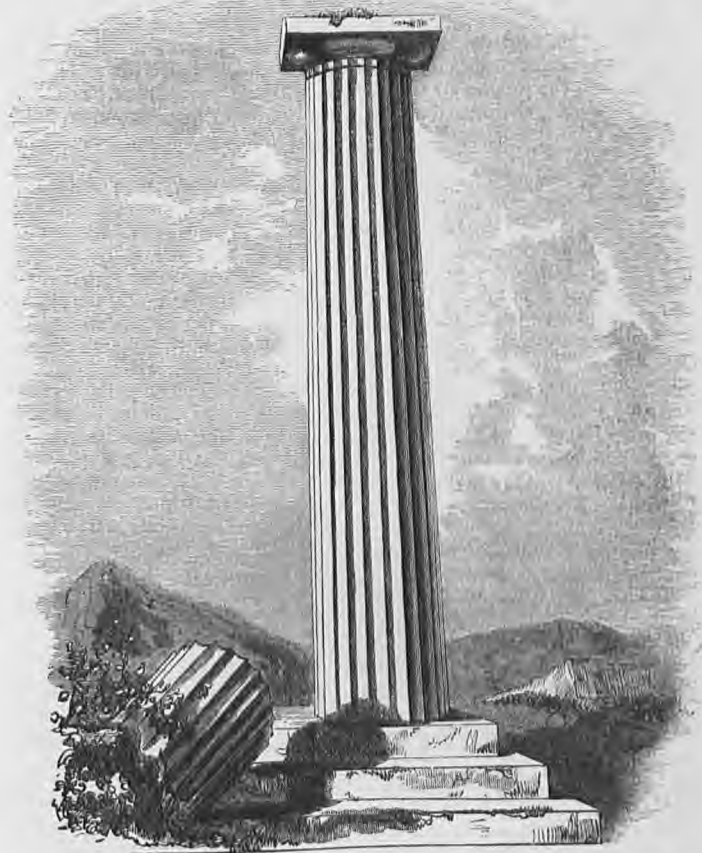
Fig. 12. A Grecian Doric Column, for Comparison with a Sigillaria Stem (p. 17)
