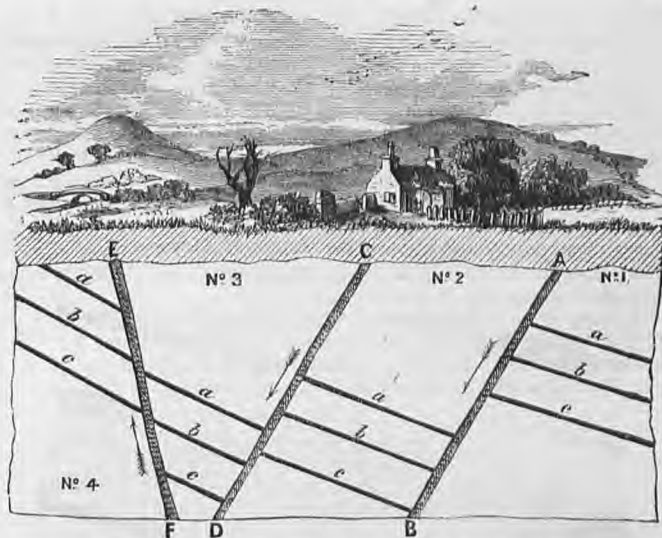
Fig. 30. Slips, or Faults. The arrows show the direction of the down-throw and up-throw.
