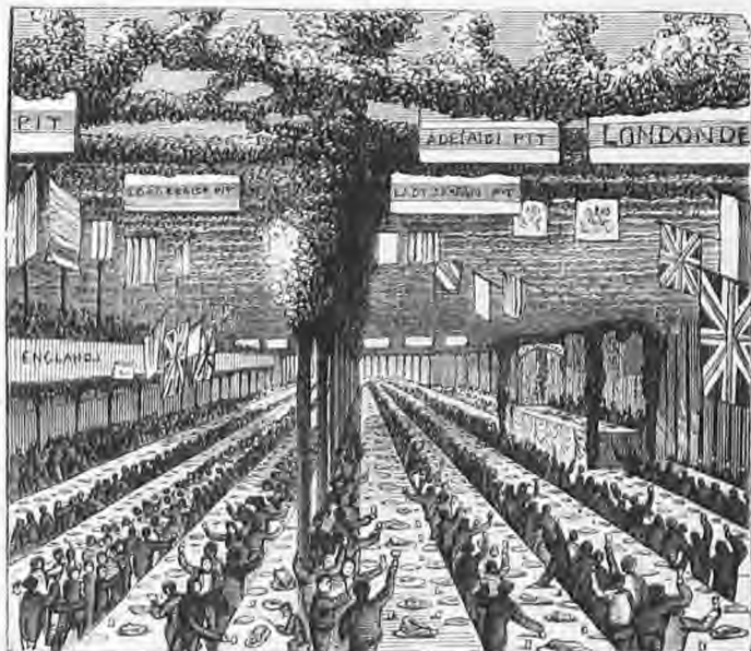
Fig. 65. The Marchioness of Londonderry's Banquet to the Workmen and Miners engaged in her Coal Fields.
