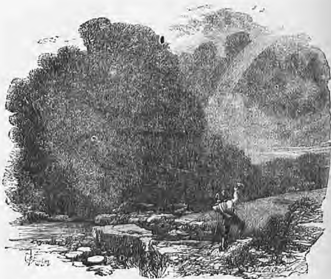
Fig. 241. The Rainbow, which is typical of the multiplicity of colours obtained from metals.
