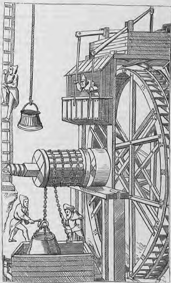
Fig. 164. Mouth of a Copper Mine, with simple mode of reversing motion of the chain on the shaft by two overshot water-wheels, (Agricola.)
