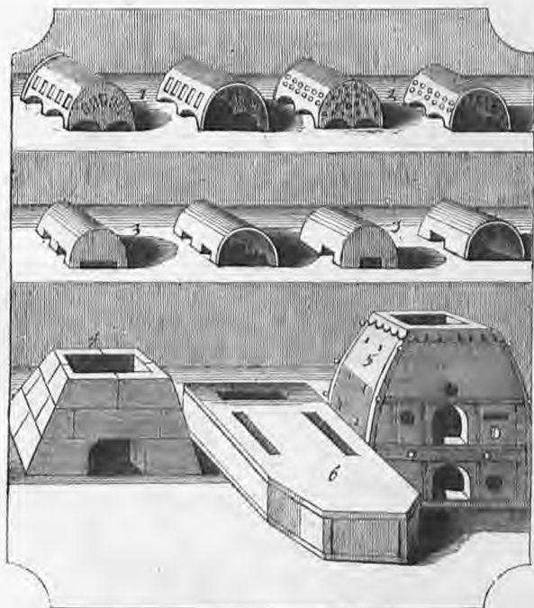
Fig. 137. "Nos. 1, 2, 3. Different forms of muffles. No. 4. An assay oven made of tiles joyned together, which may quickly be done. No. 5. An assay oven made of armour plate. No. 6. The foot of it." (Pettus.)
