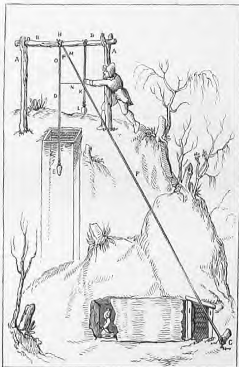
Fig. 147. The Adit Level. A, A. Two uprights or yokes supporting a bearer n n. c. The well, pit, or shaft. D. First cord. E. Weight of the first cord. F. The second cord, fixed to the earth at g. H. Head or ends of cords. I I. The mouth or entrance of the adit or tunnel. K. The third cord, with weight attached, L. M. The first measure; N, the second; O, the third, forming the triangle x. (Agricola)
