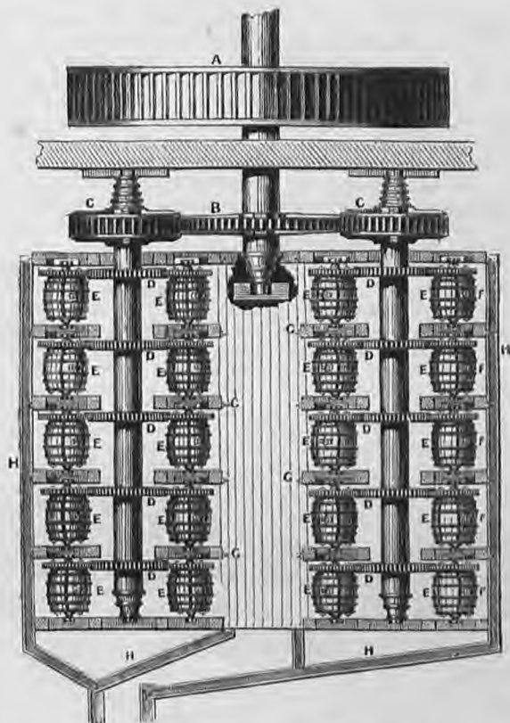
Fig. 133. Amalgamation Barrels. A is the moving wheel; a is another wheel, with 108 teeth on the axle of A ; c , c are smaller cog wheels, working to correspond with a , and each of the axles on which they are placed gives motion by means of cog wheels marked b , to a number of amalgamating casks marked e , which are all provided with a half-circular piece of iron marked v , used in conjunction with a screw, to secure the opening of the cask after the materials are put in; g , g , g , g , are also screws, the purpose of which is to enable the workmen to move any of the casks from the contact of the teeth of the wheels marked d , so that it may be worked at without stopping the movements of the other casks; h , h , h , h , indicate the iron gutter which serves to convey the mercury into any one of the casks at pleasure; they are composed of several pieces, which can be moved in any direction. In general there are 20 casks in a set, each of which contains about 300 lbs., or 30 gallons of water, and about 1000 lbs. of the decomposed mineral and pieces of scrap or forged iron. The casks are fastened up and rotated for about an hour; 500 lbs. of mercury are then put into each cask, and it is firmly closed. The machinery is so regulated as to permit the casks to turn round about fifteen or twenty times in a minute. Every four hours the amalgamation is examined, and in about sixteen hours the operation is completed.
