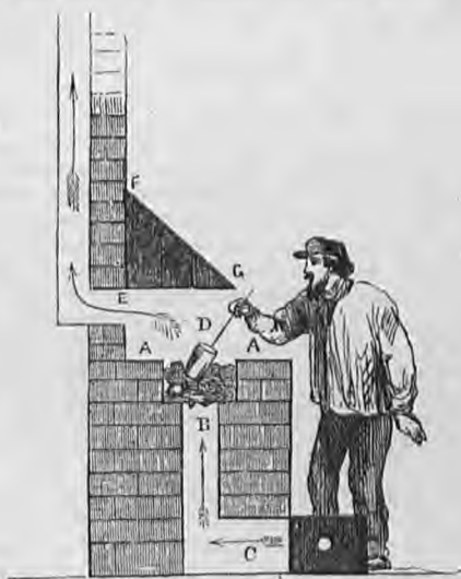
Fig. 169. Roasting Furnace. A A. A square cavity in brickwork, with small grate at B , to which air passes from the opening C , closed at pleasure by a door and register. D. The crucible containing the powdered "matt," which is kept at a very low heat, and occasionally stirred with a steel rod; the sulphur is oxidized and carried up the chimney at E , and the whole is covered with a hood of sheet iron, F G .
