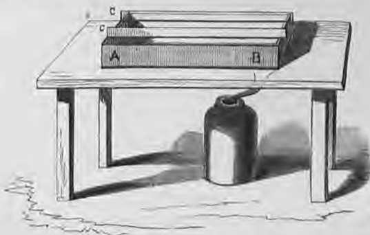
Fig. 140. A B. The gutta-percha trough and pipe leading to the stone jar containing zinc. C, C. Two glass plates levelled on the top of the trough, to carry the glass plates for developing.
