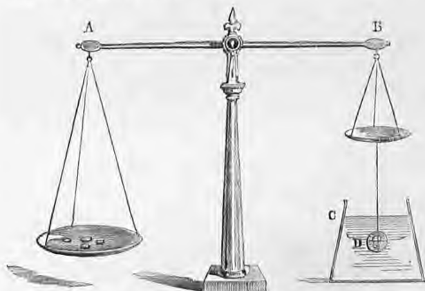
Fig. 123. Mode of taking the Specific Gravity of a Sovereign. A. B. The delicate balance. C. Vessel containing distilled water. D. The sovereign suspended by a horse-hair.
