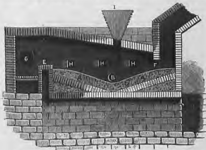
Fig. 155. Section of the Reverberatory Furnace used for roasting and smelting Galena. A. The hearth or sole of the furnace. B. Tap hole. E. The bridge which separates the fire from the hearth upon which the ore is placed. F. The flue. G. Hole through which the fuel is placed in the fire below. H, H, H. Openings, closed by sliding iron plates, for the admission of air. I. The hopper by which the ore is passed into the furnace.
