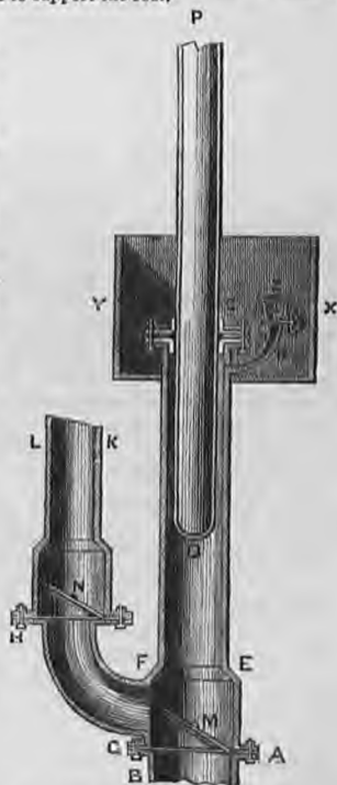
Fig. 193. The Plunger Force-pump.
