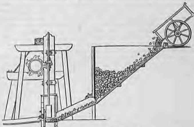
Fig. 176. Modern Stamping Mill. (Henderson.)
