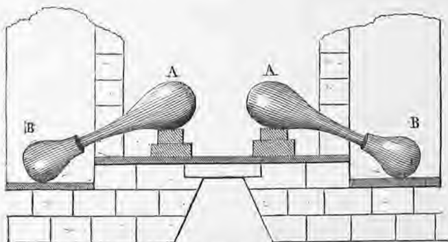
Fig. 74. A, A. Cureubites containing Mercurial Ore. B, B. The Receivers half full of Water.
