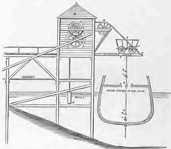
Fig. 67. One of the Forms of Staith Machinery.
