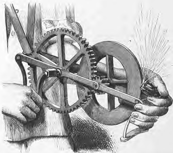
Fig. 59. The Steel Mill for giving Light in Coal Pits. The mill is attached to the waist of a boy, who holds the flint in one hand against the steel wheel, which is rapidly rotated by the other hand.
