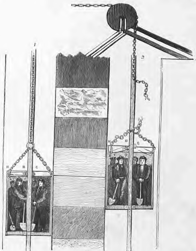
Fig. 40. Aytoun's Patent Safety Cage. 1. Cage descending and chain unbroken. 2. Chain broken, catch disengaged, and the cage stopped by the shoes or slides biting into and fixing themselves on the guide-rod.
