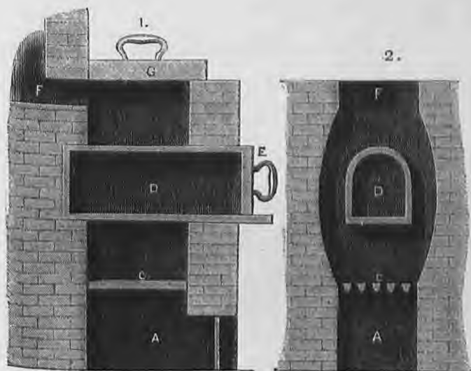
Fig. 133. Nos. 1 and 2, cupelling or enamelling furnace. In both A is the ash-pit, C the fire-bars, D the muffle, E the opening for introducing the muffle, F the chimney, and G the cover.
