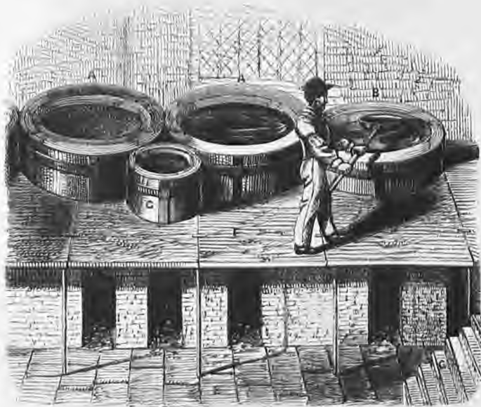
Fig. 134. Pattinson's Process. A & B , iron pans containing the argentiferous lead. C , melted lead to keep the ladle hot.
