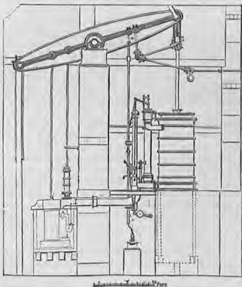
Fig. 189. A Cornish Pumping Steam-engine. (Bourne.)
