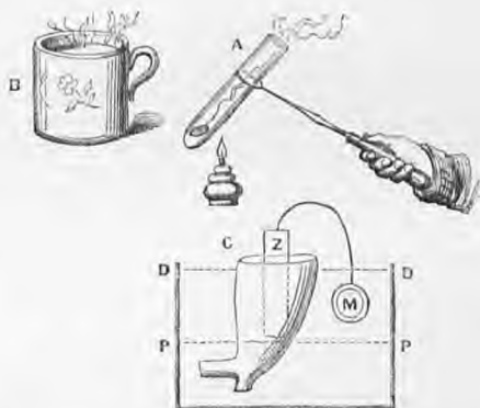
Fig. 143. A. The test tube containing the threepenny piece and nitric acid. B. Mug containing boiling water with a small quantity of hydrochloric acid. C. The gallipot with bowl of tobacco-pipe set upright in plaster of Paris (r r), and containing the dilute sulphuric acid and zinc (z). D. Solution of silver surrounding the bowl of the tobacco-pipe, and containing the article to be silvered (M).
