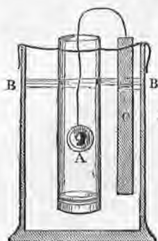
Fig. 125. De la Rive's Process of Gilding. A. Lamp chimney closed at the lower end with bladder containing the solution of chloride of gold; it is supported so that the bladder end does not touch the bottom of B B, the outer vessel, containing the acidulated water. C. The plate of zinc attached by a wire to the article which is to be gilt.
