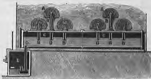
Fig. 185. A, A. The retorts. The pipes leading from the retorts marked n. c. c. The condenser of cast iron nearly filled with water into which the pipes n dip. d. Pipe through which the condensed mercury falls into the iron chest x, which is provided with a float and rod to indicate the quantity of condensed mercury.
