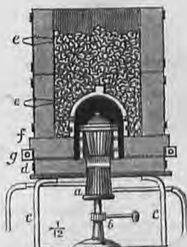
Fig. 212. Gas Furnace with Gas Jet at the Bottom.
