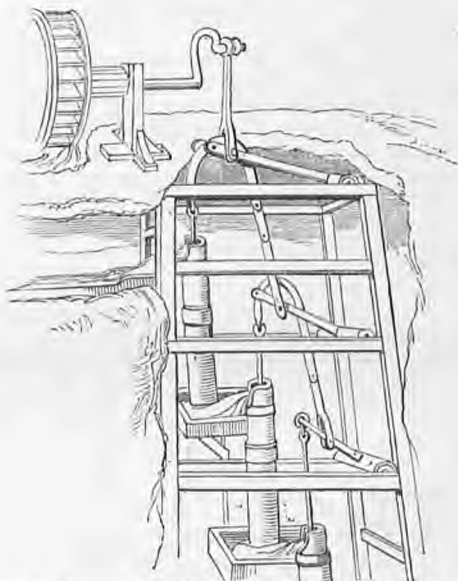
Fig. 200. Pumping Apparatus used three hundred years ago. (Agricola, 1550.)
