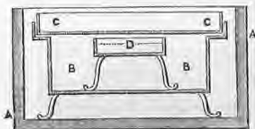
Fig. 186. Apparatus for freezing Mercury.
